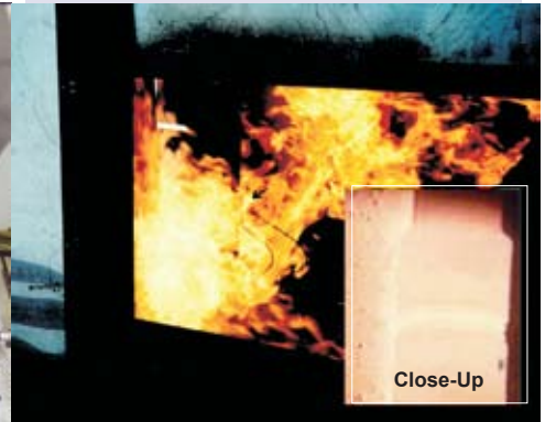
Figure 3: Fire Testing
