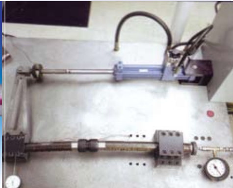
Figure 2: Fatigue testing
